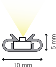
CROSS SECTION PROTECTIVE CASING
