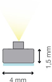
CROSS SECTION
